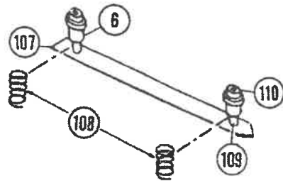
Assembly 252X, Fold Adjustment Assembly WRA095102
