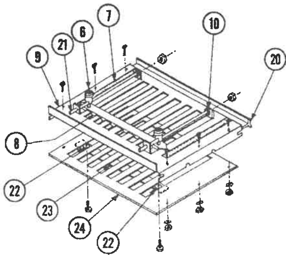
Assembly 251X, Upper and Lower Fold Tables Complete - WRA095101
