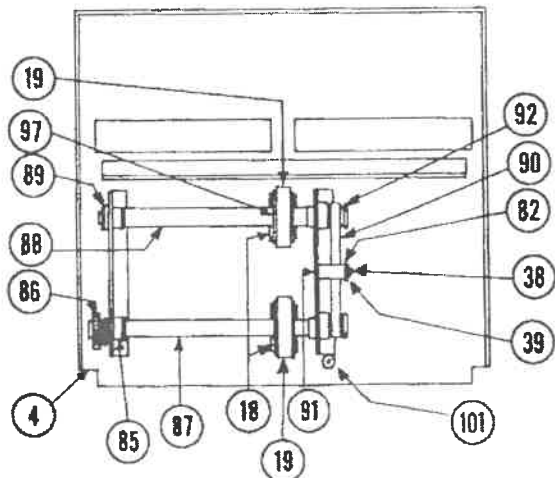
Food Table 354X Parts Detail
