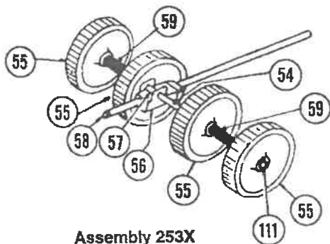
Assembly 253X Stacking Wheel Assembly WRA095103
