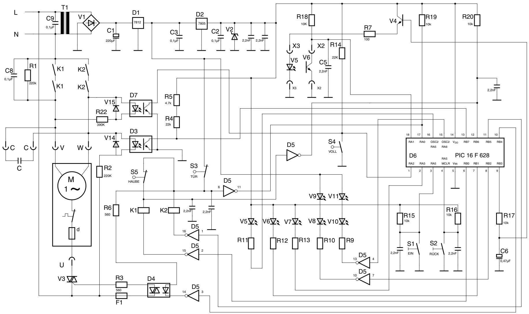
Stromlaufplan 2404 A schema de circuit electric 2404 A wiring diagram 2404 A
