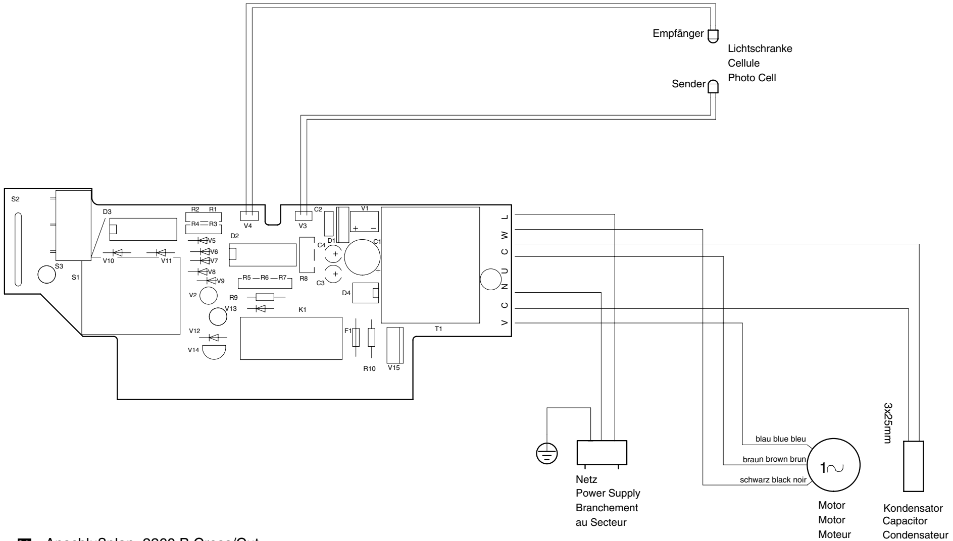
Anschlußplan 2260 B Cross/Cut Diagramme de branchement 2260 B Cross/Cut Connecting diagram 2260 B Cross/Cut
