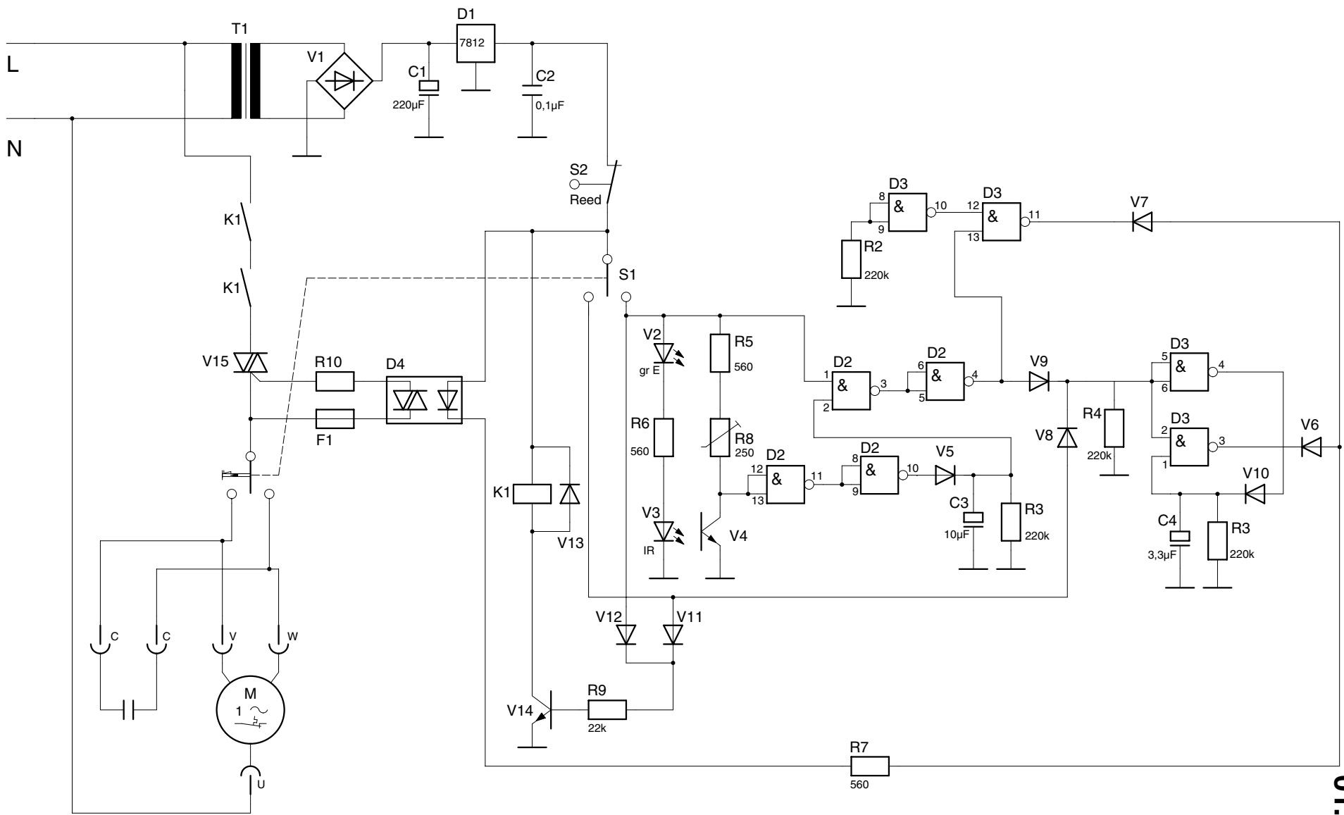
Stromlaufplan 2260 B Cross/Cut schema de circuit ectrique 2260 B Cross/Cut wiring diagram 2260 B Cross/Cut
